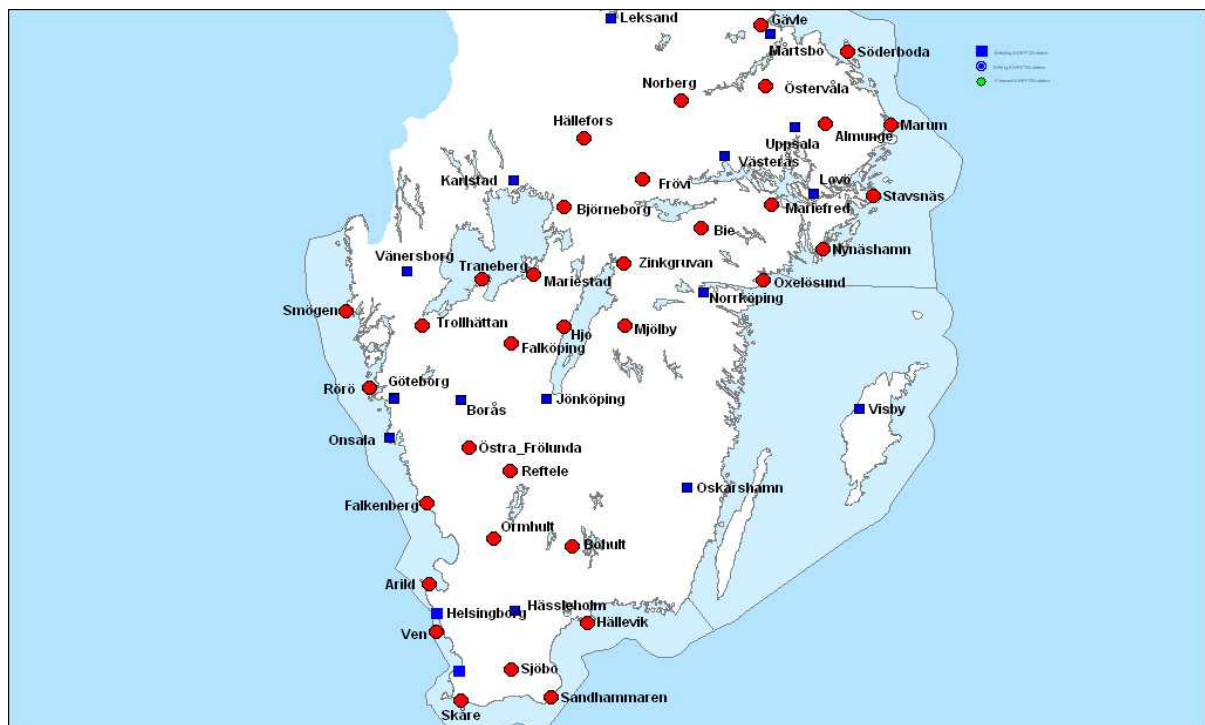
Fig. 8 Older SWEPOS stations (squares) and new RTK stations (rings) in the Southern half of Sweden (autumn 2002).
