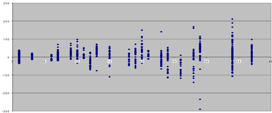
Fig. 6. Vertical deviations (mm) as function of distance (km) to nearest reference station (893 meas. 15 out.)
