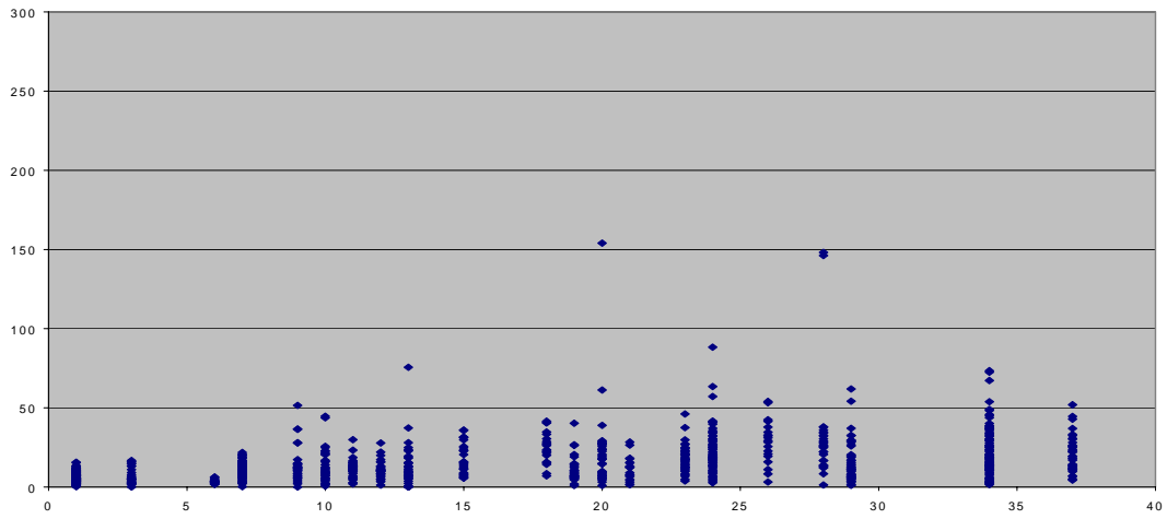
Fig. 4. Horizontal deviations (mm) as function of distance (km) to nearest reference station (970 meas., 20 out)
