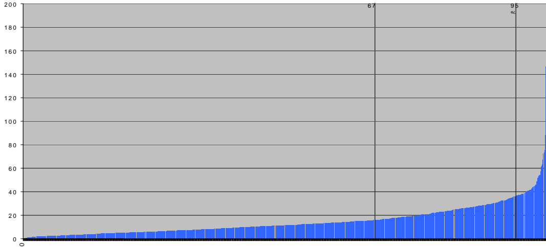
Fig. 3. Horizontal deviations (mm), sorted in order of size, 970 measurements, 20 outliers
