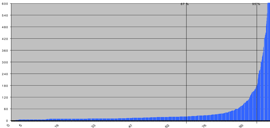
Fig. 7. Initialisation times (sec) sorted in order of speed (970 meas 20 out.)
