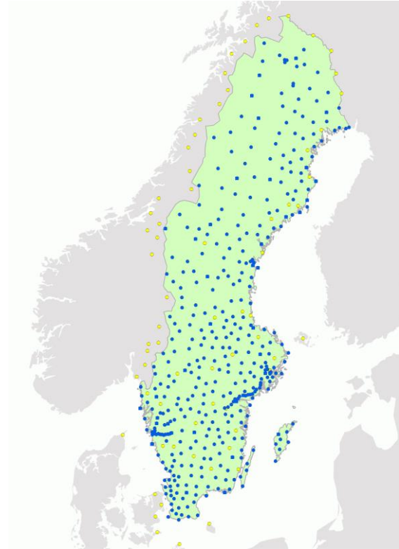
Figure 4.3: The SWEPOS network in May 2018. Squares indicate class A stations and dots indicate class B ones. Stations in neighbouring countries as well as stations from other service providers in Sweden used in the SWEPOS Network RTK Service are also marked.
